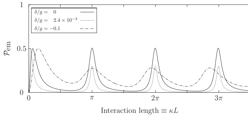
FIG. 5 – Photon emission probability in the cold atom regime ( k/\kappa = 0.05 ) for different detuning values and in the case of a mesa mode function.
